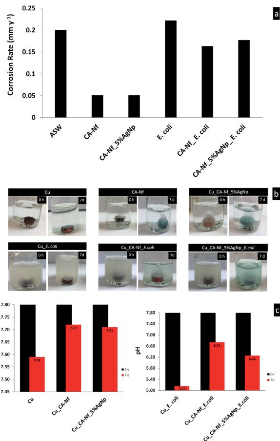
Fig. 7 Cu, Cu coated CA-Nf and Cu coated CA-Nf with 5% AgNps in the ASW and ASW inoculated with E. coli for 7 days. Also, Fig. 7 shows photographs of the Cu discs weight loss analysis in ASW and ASW inoculated with bacterium. It obviously shows that the corrosion rates decrease with the presence of CA-Nf coatings in both ASW and ASW inoculated with bacterium. The observed decreased corrosion rates are associated with larger surface
