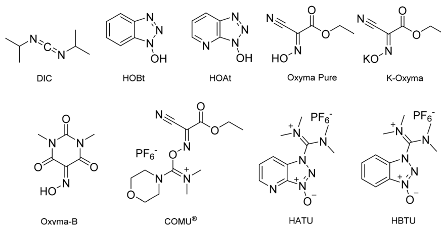
Fig. 2 Chemical structures of peptide coupling reagents and additives commonly employed in solid-phase peptide synthesis.
