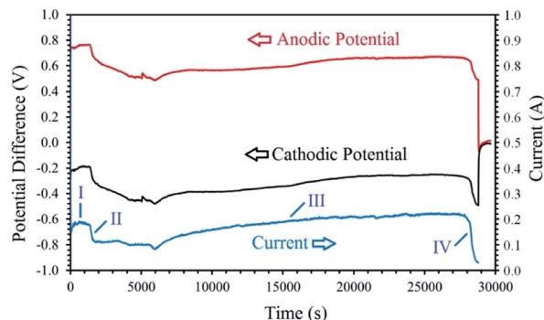
Fig. 5 The changes of cell current and cathodic/anodic voltages measured versus electrolysis time during the electrolysis of LiCl at 1 V using a cobalt oxide pellet wrapped with Ni wire served as the cathode, and a graphite crucible served as the anode under humid Ar flow. The cathodic and anodic potential differences were measured between the cathode/anode and a Mo pseudo-reference electrode immersed in the melt. 99
