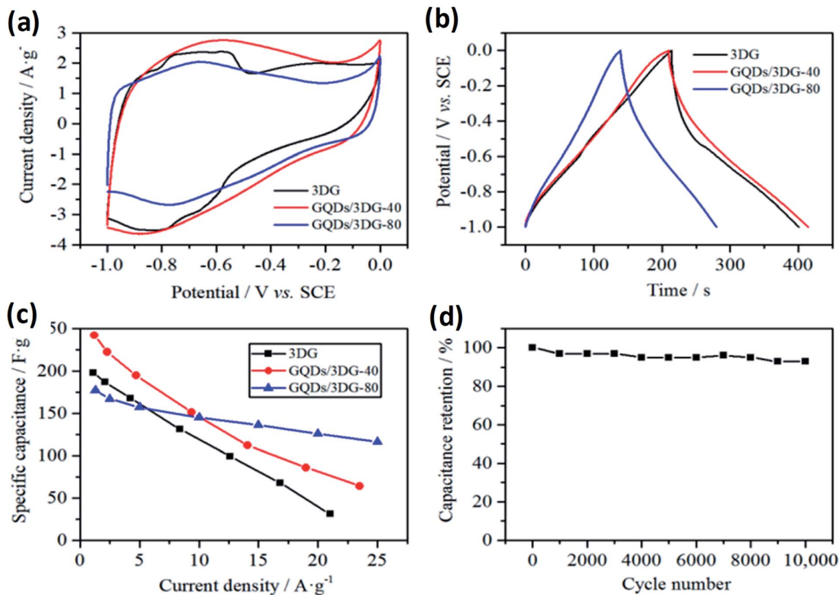
Fig. 18 (a) Cyclic voltammogram at a scan rate of 10 \text{ mV s}^{-1} (b) charge/discharge curves at different current densities with different compositions, respectively (c) specific capacitance versus current densities and (d) cycling stability at a current density of 24 \text{ A g}^{-1} for the composite material. Adapted from ref. 183, copyright 2019, MDPI publications.
