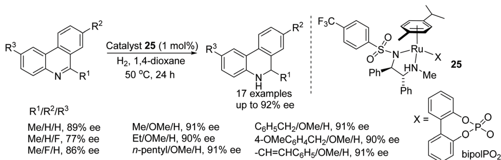
Fig. 34 Ruthenium catalyzed asymmetric reduction of phenanthridine derivatives.
