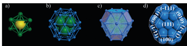
Fig. 4 (a) The central \text{Ag}_6 octahedron with a central sulfur; (b) and (c) the \text{Ag}_6\text{S}@\text{Ag}_{32} kernel; and (d) the crystal facets of the FCC \text{Ag}_{38} kernel. S yellow, Ag other colors. Adapted with permission from ref. 67. Copyright 2018, John Wiley & Sons, Inc.
