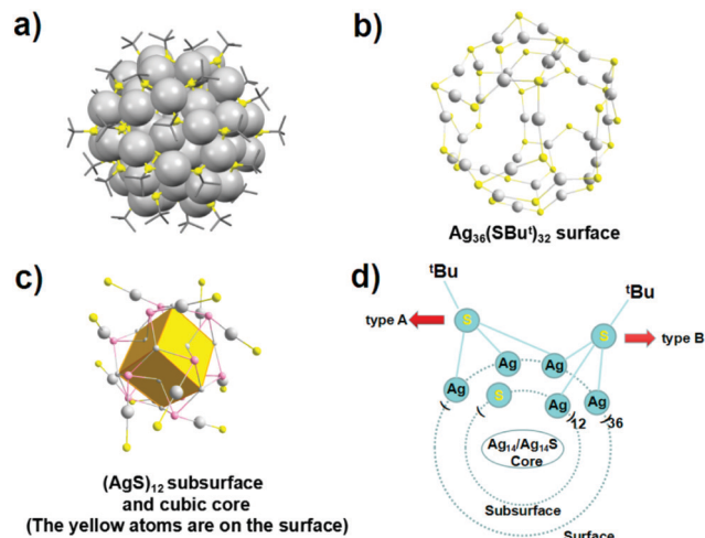
Fig. 3 X-ray structure of [\text{Ag}_{62}\text{S}_{13}(\text{S}^t\text{Bu})_{32}]^{2+} . (a) The similar frameworks contained in the Ag-QD, Ag-inter, and Ag-NC. (b) \text{Ag}_{36}(\text{S}^t\text{Bu})_{32} shell. (c) Bonding mode of core silver atoms (gray) and sulfur atoms (pink) linked with the shell sulfur atoms (yellow). (d) Two types of ligands. Adapted with permission from ref. 66. Copyright 2016, American Chemical Society.
