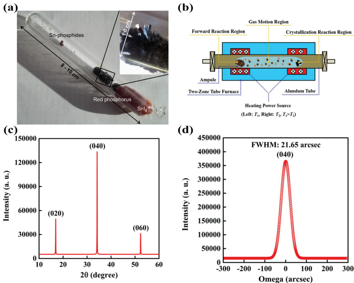
Fig. 3 (a) A silica ampule containing CVT grown BP. (b) Schematic of a tube furnace with two independent heating zones for the CVT reaction. Reproduced with the permission. (c) XRD of a BP single crystal prepared by CVT. (d) X-ray rocking curve of BP. Reprinted with permission from ref. 27 and 29. Copyright 2014 Elsevier and 2016 Springer-Verlag, respectively.
