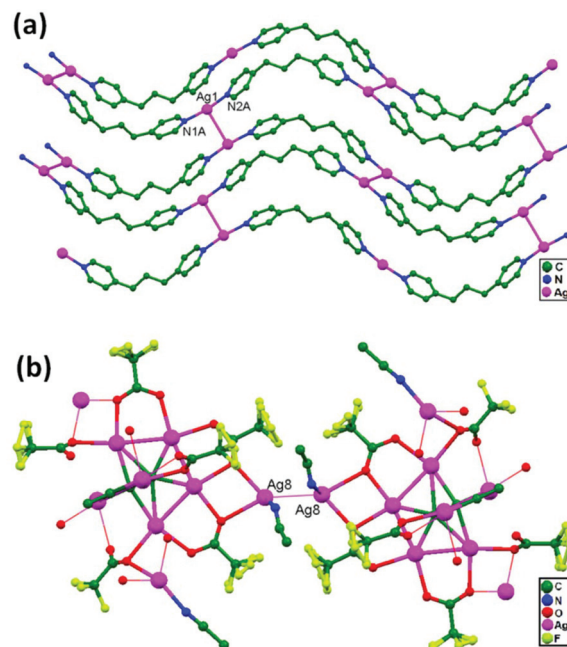
Fig. 13 (a) A 2D polymeric chain formed via Ag–Ag contacts in [Ag(\text{bpp})]ClO_4 , 17 ; ClO_4^- counter anions and hydrogen atoms are removed for clarity. (b) Strong ligand-unsupported Ag8–Ag8 interactions in Ag_2C_2 \cdot 6CF_3CO_2Ag \cdot 3CH_3CN , 19 , resulting in the construction of a 2D network.
