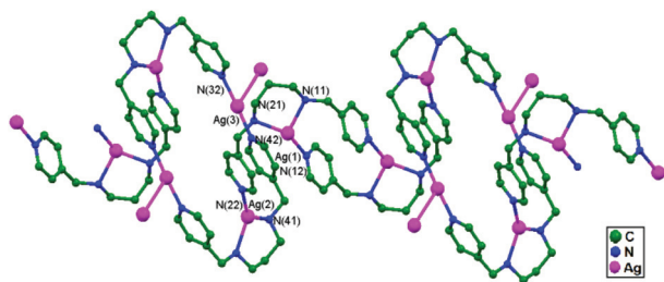
Fig. 12 The coordination environment of two-coordinate Ag^+ ions in [Ag_3(\text{py-hep})_2](ClO_4)_3 \cdot 0.5CH_3CN , 16 , and the formation of a brick-wall network via weak ligand-unsupported Ag–Ag interactions.
