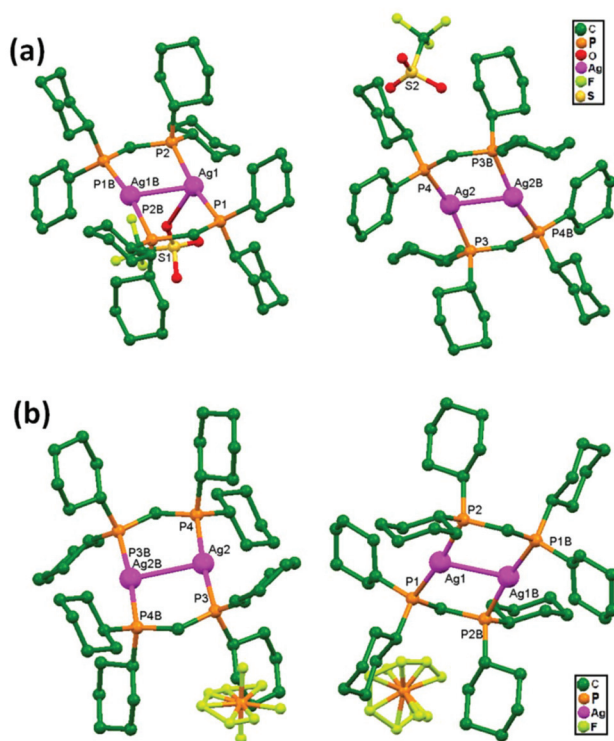
Fig. 11 Perspective views of [Ag_2(\mu\text{-dcpm})_2]X_2 (where X = CF_3SO_3 for (a) and PF_6 for (b)); the anions CF_3SO_3 and PF_6 are present in the lattices of compounds 14 and 15 , respectively.
