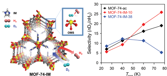
Fig. 11 Selectivity of MOF-74-IMs as function of exposure temperature ( T_{\text{exp}} ) after exposure to 1:1 \text{H}_2/\text{D}_2 mixture. Here, OMS is open metal site. Reproduced with permission from ref. 87. Copyright 2017, American Chemical Society.
