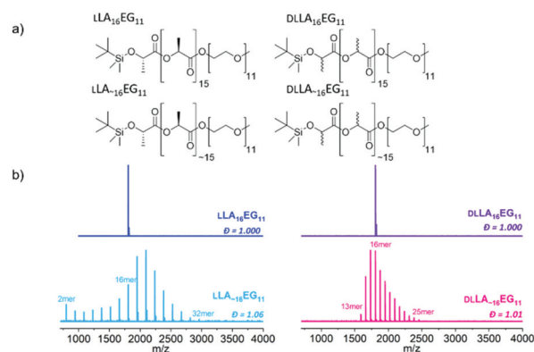
Fig. 1 (a) Chemical structures of studied BCOs: crystalline discrete LA_{16}EG_{11} , crystalline disperse LA_{\sim 16}EG_{11} , amorphous discrete DLA_{16}EG_{11} and amorphous disperse DLA_{\sim 16}EG_{11} . (b) MALDI-ToF spectra of all BCOs.
