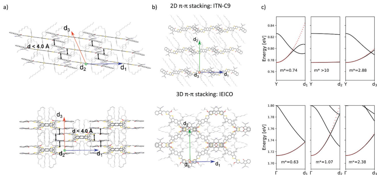
Fig. 5 (a) Lateral views of the brickwork 2D packing motif of ITN-C9 (top) and reticular 3D packing of IEICO (bottom). Black arrows represent centroid-to-centroid close contacts ( d < 4.0 Å) (b) top views of the packing structures of ITN-C9 (top) and IEICO (bottom) molecules. (c) Calculated conduction band with DFT along d_1 , d_2 and d_3 directions for ITN-C9 (top) and IEICO (bottom), effective mass values are also shown. Solvent molecules and hydrogen atoms have been omitted from panels (a) and (b) for clarity.
