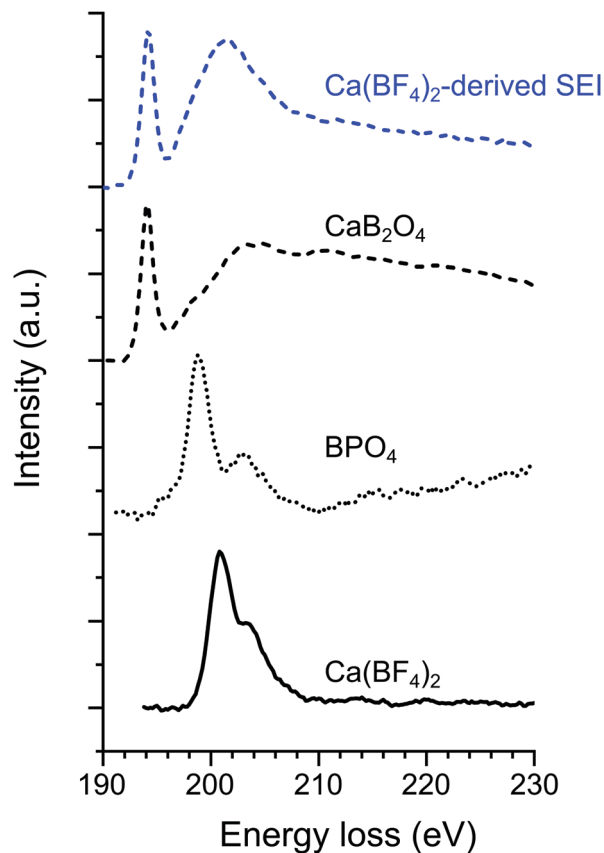
Fig. 4 Normalized EELS spectra on the B K-edge for the \text{Ca}(\text{BF}_4)_2 -derived passivation layer (“SEI” deposit shown in Fig. 1c) together with three boron-containing compounds serving as references i.e. , \text{CaB}_2\text{O}_4 , \text{BPO}_4 , and \text{Ca}(\text{BF}_4)_2 .
