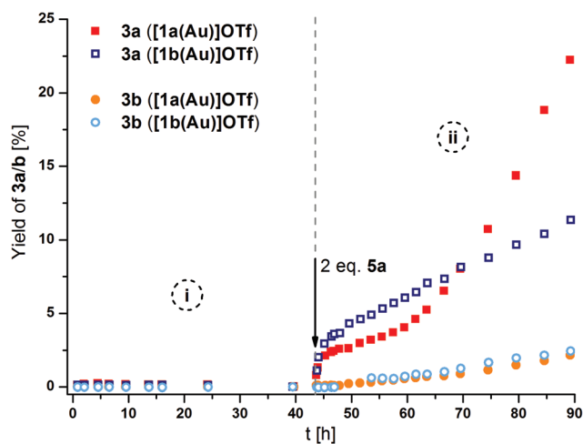
Fig. 10 Reaction profiles for ring-closing isomerisation of 2 to 3a (squares) by [\text{1a}(\text{Au})]\text{OTf} (solid symbols) and [\text{1b}(\text{Au})]\text{OTf} (hollow symbols), also showing the formation of the aromatic follow-up product 3b (circles) before (i) and after (ii) oxidation with 2 eq. 5a (with respect to catalyst; 3 mol% Au, [\text{2}]_0 = 60 \text{ mmol L}^{-1} , \text{CD}_2\text{Cl}_2 , 25 °C). For corresponding ^1\text{H} NMR spectra and TOF regression plots, s. Fig. S73, S75, and S76†
