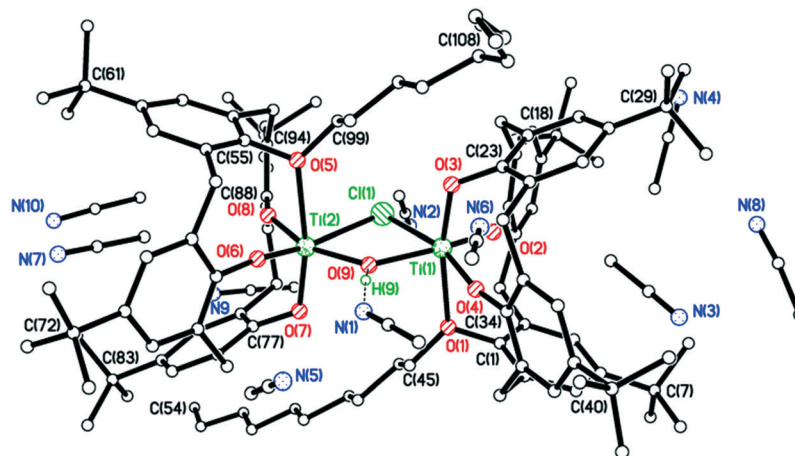
Fig. 7 Molecular structure of {[TiL(O) 3 (On-decyl) 2 (μ-Cl)(μ-OH)]·8.5MeCN (10·8.5MeCN) (most H atoms are omitted for clarity). Selected bond lengths (Å) and angles (°): Ti(1)–O(1) 2.381(3), Ti(1)–O(2) 1.817(3), Ti(1)–O(3) 1.852(3), Ti(1)–O(4) 1.793(3), Ti(1)–O(9) 2.000(3), Ti(1)–Cl(1) 2.5177(14); O(1)–Ti(1)–O(3) 168.54(13), O(2)–Ti(1)–O(4) 102.84(15), Cl(1)–Ti(1)–O(9) 74.82(10), Ti(1)–O(1)–C(1) 112.8(2), Ti(1)–O(2)–C(12) 150.5(3), Ti(1)–O(3)–C(23) 119.9(2), Ti(1)–O(4)–C(34) 168.3(3).
