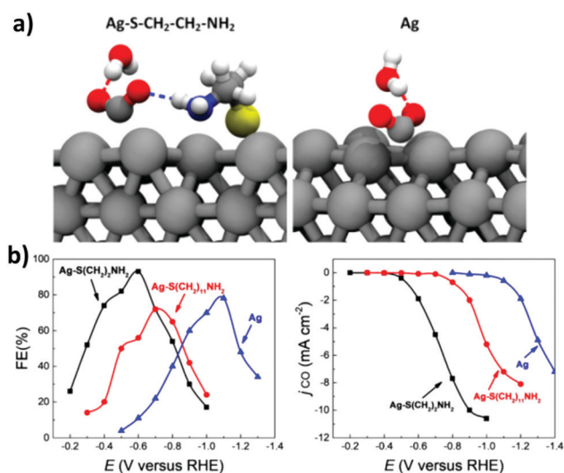
Fig. 31 (a) Chemisorbed \text{CO}_2 on cysteamine-functionalized (left) and on cysteamine-free (right) Ag(111) surface. Only the water molecules directly forming hydrogen bond (slashed line) are shown. The colors are: Ag in silver, C in gray, O in red, N in blue, S in yellow, and H in white. (b) Influence of the alkyl chain length on \text{CO}_2\text{RR} in terms of \text{FE}_{\text{CO}} (left) or j_{\text{CO}} (right) vs. potential. Reproduced with permission from ref. 419. Copyright 2018 American Chemical Society.
