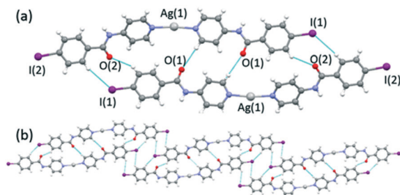
Fig. 4 (a) A view showing \text{Ag}(\text{I}) coordination in 1 and hydrogen bonded dimers and (b) ribbons formed by edge-to-edge hydrogen bonding interactions ( \text{C}_{\text{Ar}}\text{--H}\cdots\text{I} ).
