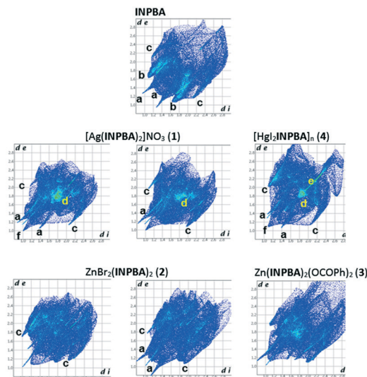
Fig. 11 Fingerprint plots of the INPBA ligands, crystallographically different in the crystal structures of INPBA and 1 to 4 .
