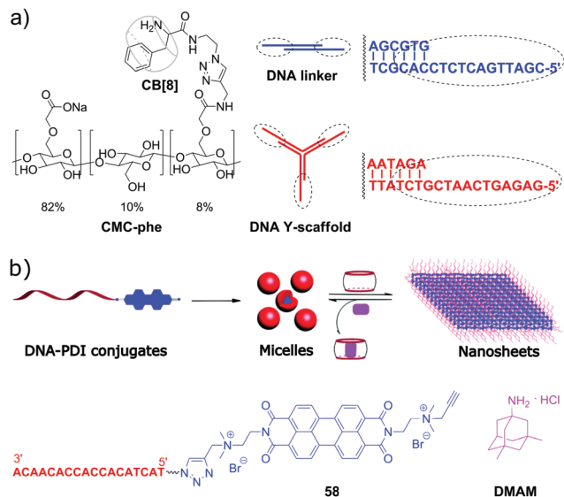
Scheme 12 (a) Molecular building blocks self-assembling into a double network hydrogel based on the interpenetrating CB[8]- and DNA-based networks; (b) structure of the ssDNA-perylenediimide conjugates, schematic representation of their self-assembly into spherical micelles and rearrangement into nanosheets upon addition of CB[10]. Adapted from ref. 95, copyright RSC.
