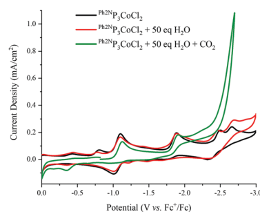
Fig. 3 Cyclic voltammograms of 1\text{ mM Ph}_2\text{N-P}_3\text{CoCl}_2 under various conditions. (Black): under \text{N}_2 ; (red): in the presence of 50 eq. \text{H}_2\text{O} ; (green): in the presence of 50 eq. \text{H}_2\text{O} and \text{CO}_2 . Conditions: GC working electrode, 0.1 M TBAPF 6 electrolyte in MeCN solvent, scan rate of 0.06\text{ V s}^{-1} , initial scan is positive.
