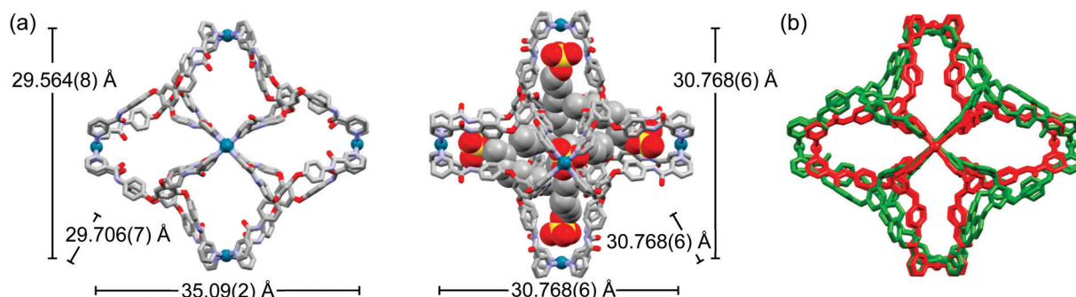
Fig. 1 Crystal structures and Pd...Pd distances for 1 \cdot 12NO_3 (a, left) and 2 \cdot C_8H_{15}OSO_3 (a, right). Overlay (b) of 1 \cdot 12NO_3 (green) and 2 \cdot C_8H_{15}OSO_3 (red).
