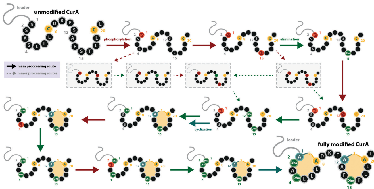
Fig. 3 Processing order of the CurA precursor peptide by the CurKC processing enzyme, which was investigated in-depth using the deuterium-labeling approach as described in the main text. 50 This case exemplifies that while a general C-to-N-terminal directionality is observed, there can be exceptions to this order (here, Ser1 is phosphorylated first) and that besides the major processing route, minor routes can be detected with sufficient scrutiny (note that only a few exemplary early minor processing routes are shown and not all that were described in the original publication 30 ). This example also emphasizes that while usually the same residue becomes phosphorylated and eliminated before the next residue is processed, there are also exceptions to this rule. pS = phosphoserine.
