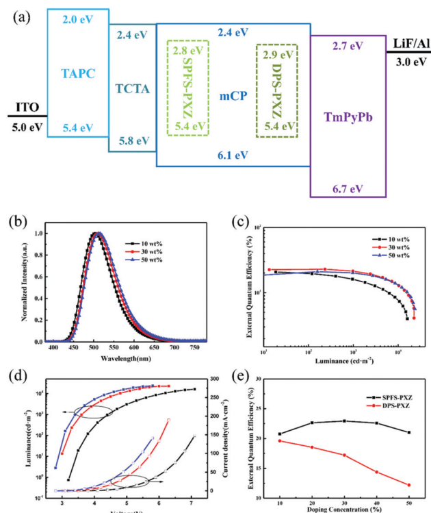
Fig. 4 (a) Energy level diagram of SPFS-PXZ -doped and DPS-PXZ -doped devices. (b) EL spectra at 1000 cd m -2 , (c) luminance-external quantum efficiency and (d) voltage-luminance-current density characteristics of SPFS-PXZ -doped devices for different doping concentrations: black (10 wt% doped in mCP), red (30 wt% doped in mCP), and blue (50 wt% doped in mCP). (e) Effect of maximum external quantum efficiency-doping concentration on mCP characteristics of SPFS-PXZ (black) and DPS-PXZ (red) based OLEDs.
