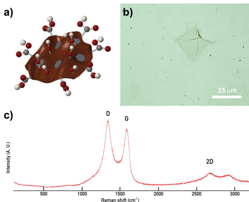
Fig. 1 Schematic representation of a GO flake and characterisation results. (a) Scheme illustrating the 2D and amphoteric nature of GO due to the configuration of different functional groups on the basal plane (carboxylic acids –COOH, hydroxyls –OH, epoxy rings –O–, and un-oxidised islands) and edges (–COOH & –OH) on GO flakes. (b) Image of a GO flake taken with an optical microscope; (c) Raman spectrum showing the characteristic vibrational peaks for GO (D, G and 2D). 27,29
