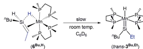
Scheme 4 Solution decomposition of [(\text{dmpe})_2\text{MnH}(\text{}^n\text{BuHSi}=\text{CHMe})] ( 6^{\text{Bu,H}} ) to form silylene complex \text{trans}-[(\text{dmpe})_2\text{MnH}(\text{SiEt}^t\text{Bu})] ( \text{trans}-3^{\text{Bu,Et}} ) as the major product.
