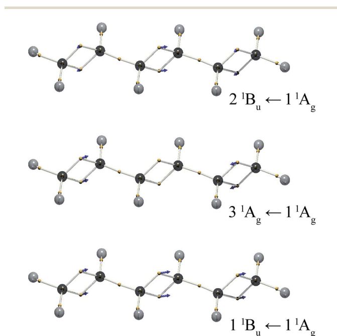
Fig. 6 The electron positions for the mid-point of the vibration, \bar{x} = (x_i + x_f)/2 , and the displacement vectors x_{fi} , for the 1^1B_u \leftarrow 1^1A_g , 3^1A_g \leftarrow 1^1A_g and 2^1B_u \leftarrow 1^1A_g transitions of trans,trans -hexatriene. The vector length is doubled for clarity.
