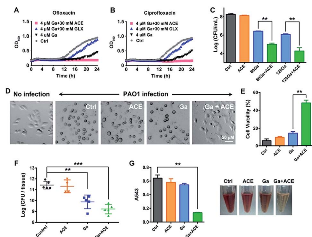
Fig. 4 Acetate enhances the antimicrobial effectiveness of Ga(III) and decreases P. aeruginosa virulence. (A and B) Growth curves of P. aeruginosa persists in the presence of Ga(III) or the combination with acetate or glyoxylate. (C) A549 cell-associated bacterial colony counts in the in vitro cell infection model. (D) Cell morphology after 4 h P. aeruginosa infection for 4 h. (E) Viability of A549 cells after 4 h P. aeruginosa infection, corresponding to data in (D). (F) CFU of P. aeruginosa counted in the infected mice tissues after treatment with the vehicle, sodium acetate (1 g kg -1 ), Ga(NO 3 ) 3 (2 mg kg -1 ) or their combinations 48 h post-infection. (G) Haemolytic activities of P. aeruginosa exposed to sub-inhibitory concentrations of acetate (10 mM), Ga(III) (6 μM) or their combination. Data are presented as mean ± SEM from biological replicates. The asterisks indicate significant difference from the Ctrl or Ga(III) treatment group (**, 0.001 < p < 0.01 and ***, p < 0.001).
