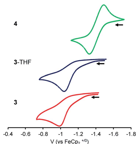
Fig. 3 CVs of 3 , 3-THF and 4 with 0.1 M [^m\text{Pr}_4\text{N}][\text{BAR}_4^F] electrolyte in DFB (scan rate of 100 mV \text{s}^{-1} ; collected under Ar).
