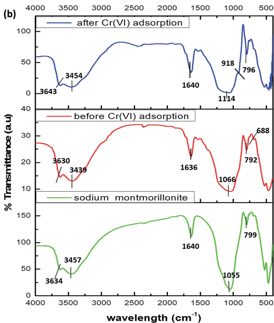
Fig. 1 (a) Calibration graph of Cr(vi) (b) FTIR of sodium montmorillonite, biosorbent before and after Cr(vi) adsorption.
