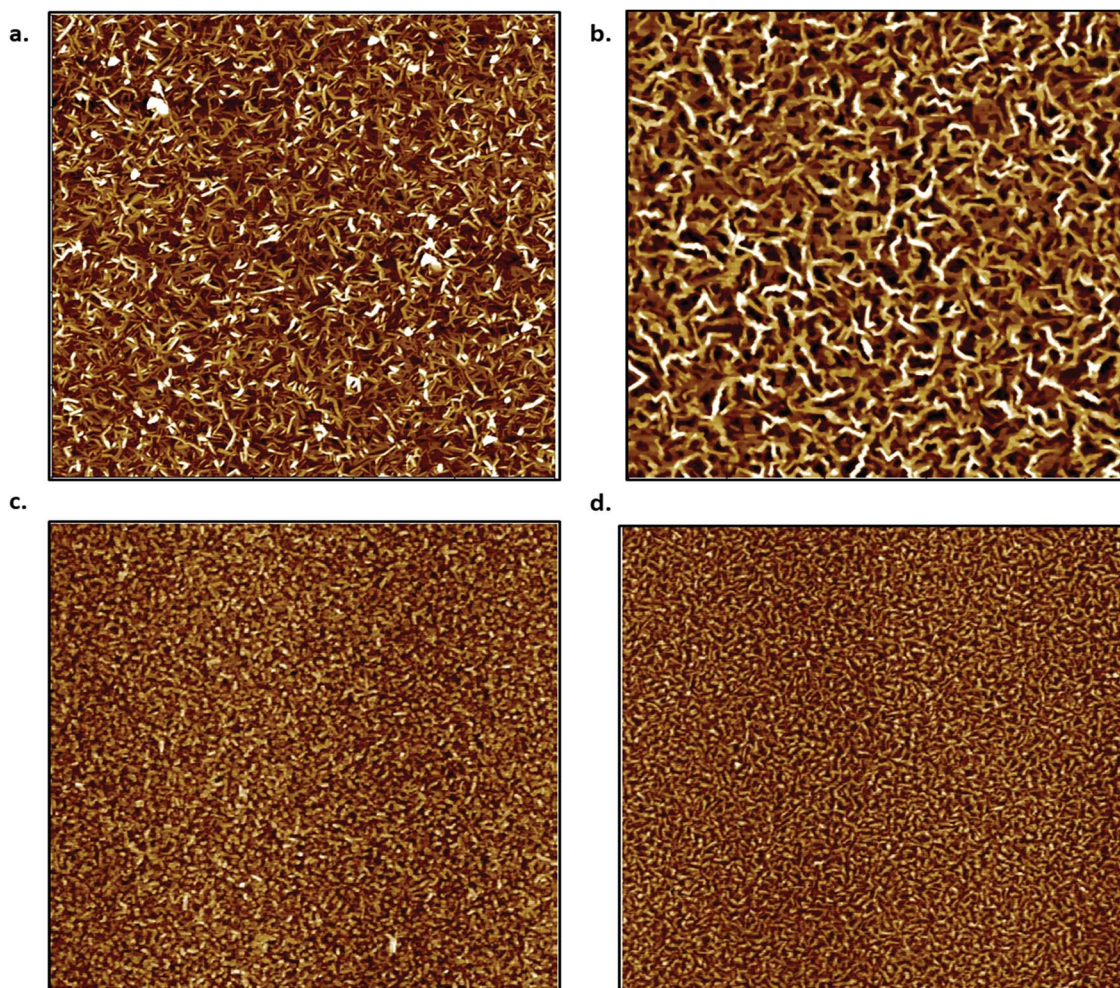
Fig. 5 AFM images of CuPc (a and c) and F 16 -CuPc (b and d) thin films deposited on SiO 2 substrates at 140 °C (a and b) and 20 °C (c and d). Images (a and b) are 5 \mu\text{m} \times 5 \mu\text{m} while (c and d) are 2.5 \mu\text{m} \times 2.5 \mu\text{m} .
