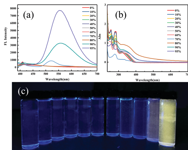
Fig. 2 (a) Fluorescence spectra and (b) absorption spectra in different THF/water (v/v) mixtures. (c) Optical images of ODFRPTZ in the mixed solution (20 μM, λ ex = 365 nm).
