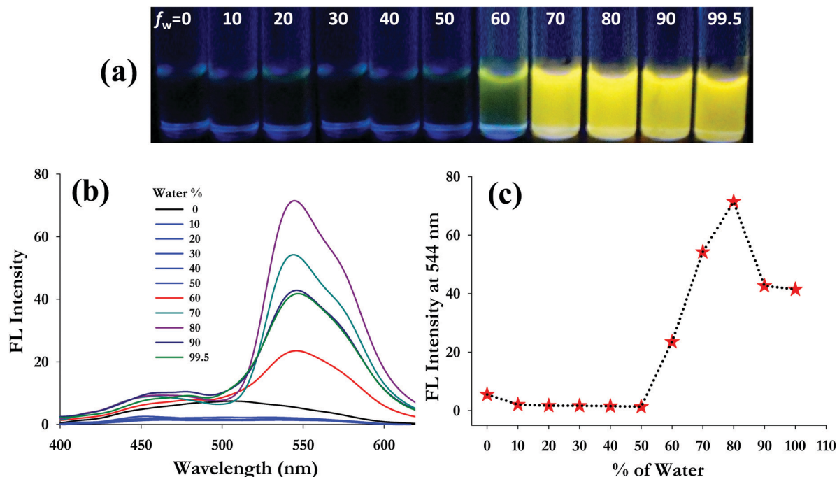
Fig. 1 (a) Visual fluorescence response of 50 \mu M probe 3 under a UV-lamp at 365 nm at varying DMSO–water (buffered by 10 mM HEPES at pH 7.4) fraction. (b) Fluorescence response for 50 \mu M probe 3 at varying DMSO–water (buffered by 10 mM HEPES at pH 7.4) fraction ( \lambda_{\text{ex}} = 362 nm). (c) Change in the fluorescence intensity of probe 3 at 544 nm as a function of different percentages of the water fraction (% f_w ).
