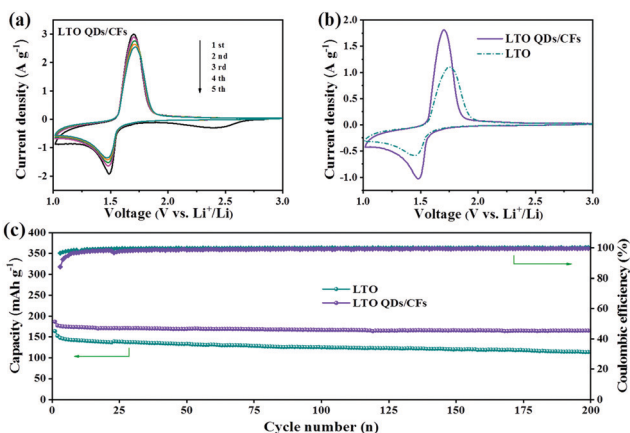
Fig. 5 (a) Five CV curves of LTO QDs/CFs at 1 mV s -1 , (b) comparison of CV curves between LTO and LTO QDs/CFs at 0.5 mV s -1 , and (c) cycling performance at 1C (1C = 175 mA g -1 ).
