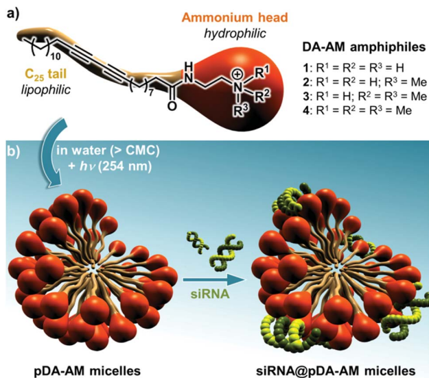
Fig. 1 (a) Structure of the four DA-AM amphiphiles; (b) micelle assembly, photopolymerization and complexation with siRNA.
