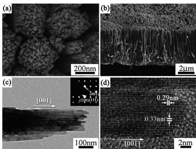
Fig. 6 (a and b) SEM, (c) TEM, and (d) HRTEM images of rutile \text{TiO}_2 nanorod arrays prepared at 150 °C on Ti foil for 20 h. The inset in (c) is the corresponding SAED pattern. Adapted with permission from ref. 64. Copyright 2012 Royal Society of Chemistry.
