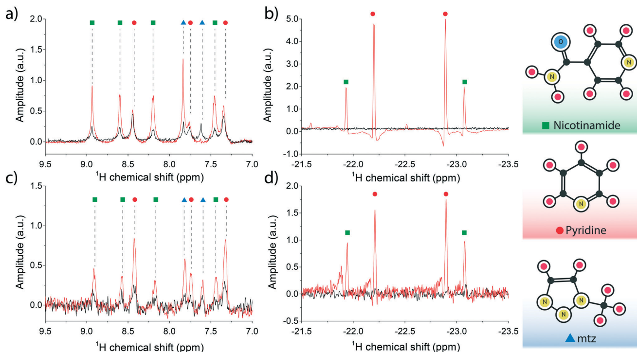
Fig. 3 (a and b) Single acquisition ^1\text{H} spectra of the SABRE mixture (25 mM pyridine, 25 mM nicotinamide, 26 mM mtz , 2.4 mM Ir-IMes catalyst) performed at B = 11.7 T and T = 30 ^{\circ}\text{C} . The SABRE measurement (in red) was recorded immediately after thoroughly bubbling the sample solution with a 90% p\text{-H}_2 enriched mixture for 20 s. The reference measurement at thermal equilibrium is plotted in black. The analyte signal peaks are shown on the left in (a), and the di-hydritic region to the right in (b). (c and d) 16-fold averaged ^1\text{H} spectra for the high-field SABRE experiment performed at B = 11.7 T and T = 30 ^{\circ}\text{C} and under active microflow conditions. The flow rate was set at the optimal value of 60\ \mu\text{L min}^{-1} . The reference measurement, in black, was recorded at rest. Peak assignment follows the colour scheme reported on the right edge of the figure, i.e. nicotinamide peaks are labelled with green dots, pyridine with red, and mtz with blue in plots (a) through (d).
