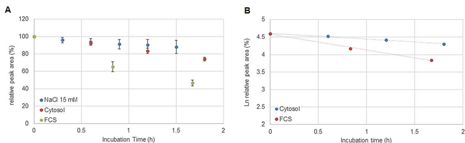
Fig. 6 (A) Stability of oxaliplatin in 15 mM NaCl assessed by RP-ICP-MS with the column Accucore PFP, 2.1 \times 150 mm, 2.6 \mu m, Thermo Scientific and stability of oxaliplatin in the cytosolic extract in N = 3 biological replicates assessed using the 2D-setup employing the column Accucore PFP, 2.1 \times 150 mm, 2.6 \mu m, Thermo Scientific compared to the previous investigated stability in FCS. The decay observed in the cytosol was different from the decay observed in 15 mM NaCl and in FCS showing a linear regression for zero order kinetics with a half-life of 3.5 \pm 0.3 h although a (B) logarithmic plot of oxaliplatin relative area versus incubation time was also observed to be linear for the investigated period for first order kinetics, as it was observed for the incubation in FCS, obtaining a half-life of 4.2 \pm 0.4 h.
