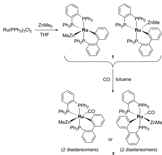
Scheme 2 Formation of [Ru(dppbz)(PPh_2(biphenyl'))ZnMe] ( 1 ) and trapping by CO.
