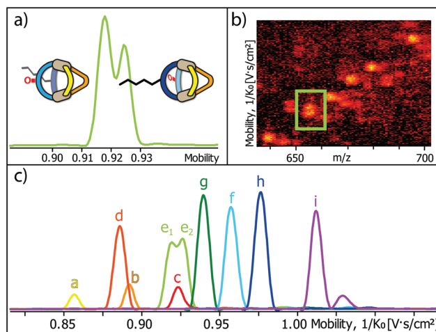
Fig. 5 (a) High resolution TIMS mobilogram allowing the discrimination of cis - [\text{Pd}_2\text{L}^{\text{C}}\text{L}^{\text{F}}\text{L}^{\text{P}}\text{L}^{\text{P}'}]^{3+} and trans - [\text{Pd}_2\text{L}^{\text{C}}\text{L}^{\text{F}}\text{L}^{\text{P}}\text{L}^{\text{P}'}]^{3+} ; (b) partial heat map and (c) full mobilogram of the simultaneous ion mobility measurement of all ten coordination cages; assignments a–i correspond to cages shown in Fig. 6.
