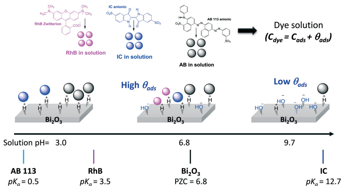
Fig. 3 Schematic of the adsorption processes of the three dyes on \text{Bi}_2\text{O}_3 at different pH values.
