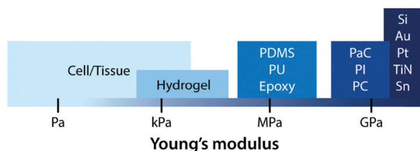
Fig. 6 Young's moduli of cell/tissue and common electrode materials. Conventional materials for electrodes are much stiffer than cell/tissue. Hydrogels exhibit a similar level of Young's moduli, potentially minimizing the mechanical mismatch with biological tissues.
