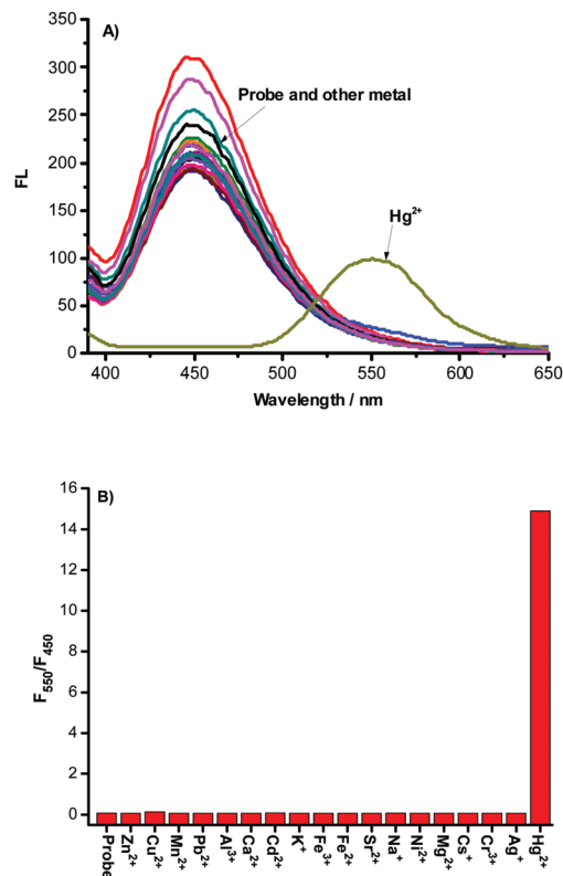
Fig. 2 (A) Fluorescence spectra of probe NAP-PS ( 10\ \mu\text{M} ) before and after the addition of 200\ \mu\text{M} different metal ions in HEPES buffer ( 1.0\ \text{mM} , \text{pH} = 7.4 ), \lambda_{\text{ex}} = 380\ \text{nm} , slits: 3/5\ \text{nm} ; (B) fluorescence intensity ratios ( F_{550}/F_{450} ) of probe NAP-PS ( 10\ \mu\text{M} ) before and after the addition of 200\ \mu\text{M} different metal ions in HEPES buffer ( 1.0\ \text{mM} , \text{pH} = 7.4 ).
