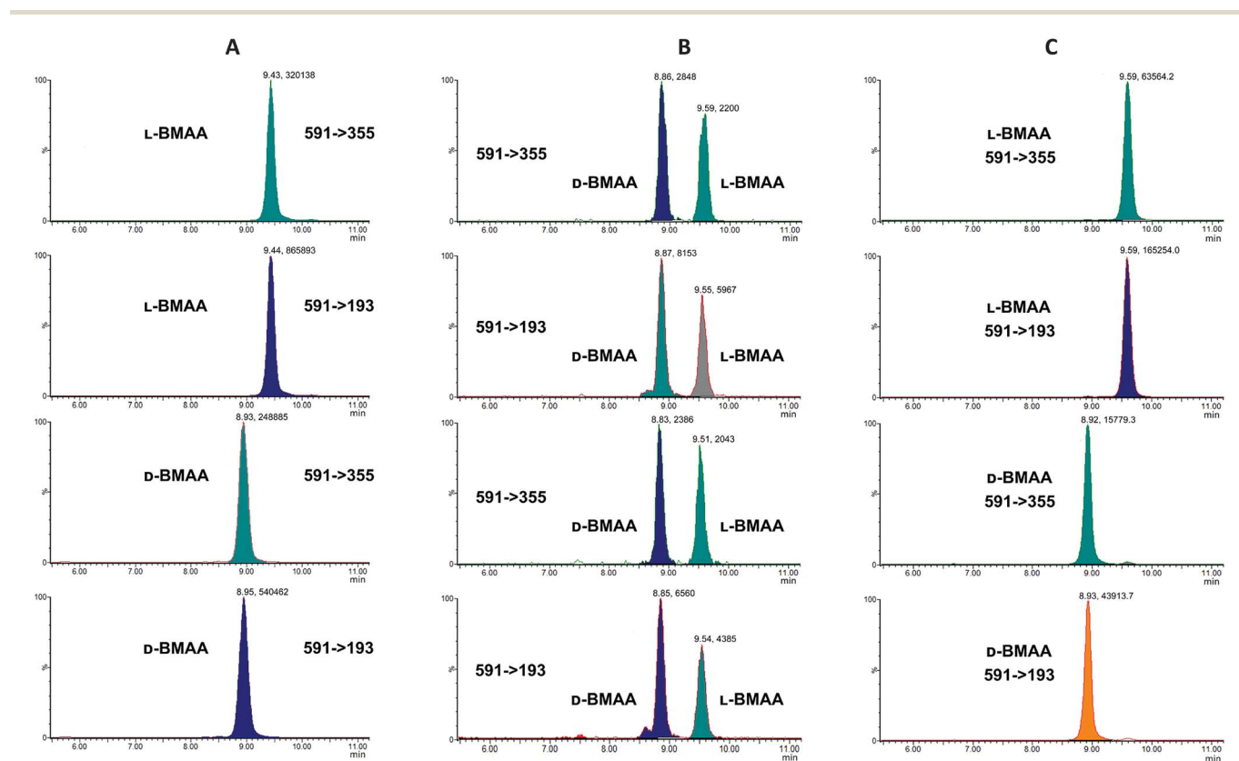
Fig. 3 MRM chromatogram of L and D standard compounds (1 mg L -1 ). Chromatograms for specific transitions corresponding to: (A) L-BMAA and D-BMAA standard solutions; (B) L-BMAA and D-BMAA standard solutions after acid hydrolysis show that racemization of L- and D-BMAA pure enantiomers occurs; but in (C) L-BMAA and D-BMAA standard solutions after enzymatic hydrolysis do not racemize, and stereochemistry of L- and D-BMAA pure enantiomers is preserved.
