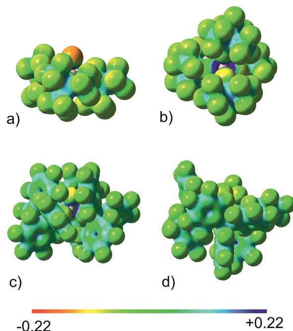
Fig. 5 Projection of the calculated electrostatic potential on the 0.025 e^- \text{ bohr}^{-3} isodensity surface. (a) [\text{FAI}(\text{OC}(\text{CF}_3)_3)_3]^- ; (b) [\text{Al}(\text{OC}(\text{CF}_3)_3)_4]^- ; (c) [\text{FAI}(\text{OCAr}^{\text{F}}_3)_3]^- ; (d) [\text{CIAI}(\text{OCAr}^{\text{F}}_3)_3]^- . B3LYP/6-311++G(2d,2p) level of theory.
