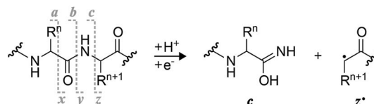
Scheme 1 Complementary c and z' fragments from N–C \alpha backbone bond cleavage between residues n and n + 1 in ECD, niECD, or ETD; z' fragment structures were confirmed by infrared ion spectroscopy, 22 c fragments with imidic acid structure can tautomerize to the amide form, 23 and H + transferring from a c to its complementary z' fragment can produce a pair of complementary c' and z fragments. 24,25
