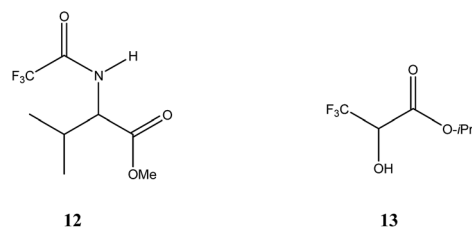
Fig. 1 Structures of N -trifluoroacetyl valine methyl ester ( 12 ) and isopropyl (3,3,3-trifluoro)lactate ( 13 ).
