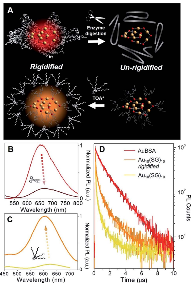
Fig. 3 Photoluminescence properties of \text{Au}_{10}(\text{SG})_{10} and AuBSA clusters in rigidified and un-rigidified states. (A) Scheme of un-rigidifying AuBSA clusters with enzyme digestion and rigidifying \text{Au}_{10}(\text{SG})_{10} clusters with \text{TOA}^+\text{I}^- toluene phase-transfer. (B) Resultant luminescence decrease of AuBSA clusters (un-rigidified, dark red line) and (C) luminescence enhancement of \text{Au}_{10}(\text{SG})_{10} clusters (rigidified, orange line). (D) Photoluminescence decay lifetime traces of AuBSA clusters (red), rigidified \text{Au}_{10}(\text{SG})_{10} clusters (orange) and original \text{Au}_{10}(\text{SG})_{10} clusters (yellow).
