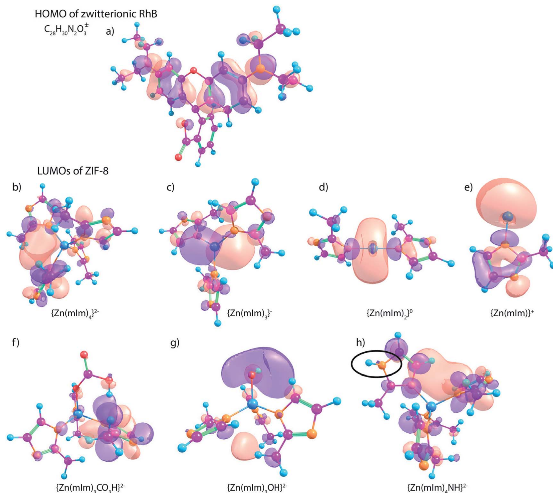
Fig. 5 DFT computationally predicted HOMO of the zwitterionic RhB ion (a) and LUMOs of ZIF-8 (b–h). ZIF-8 is represented by a cluster of \{Zn(mim)_x\}^{(2-x)} with x is an integer from 4 to 1 (model (b) to (e)). Model (f) and (g) refer to the ZIF-8 external surface groups of hydrogencarbonate and hydroxide, respectively. The surface secondary amine group is represented by model (h) with an -NH- moiety on one mim ligand, highlighted in a black circle. Carbon (purple), hydrogen (blue), nitrogen (orange), zinc (azure), and oxygen (red); positive and negative lobes are presented by orange and purple color with an isosurface value of 0.03.
