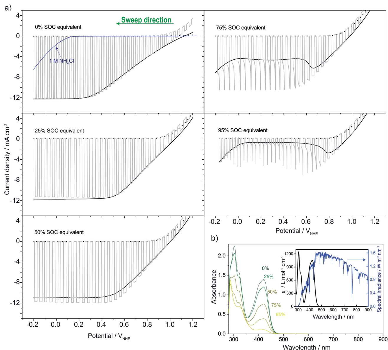
Fig. 5 (a) LSVs recorded on \text{pn}^+\text{Si}/\text{TiO}_2 in 0.4 M ferri/ferrocyanide solutions in ratios matching that expected for different SOC in the solar flow battery (SOC equivalents) and of the pure supporting electrolyte (1 M \text{NH}_4\text{Cl} displayed with the 0% SOC equivalent, blue line) relative to a reference electrode. Recorded in constant light (1 sun, full black line), chopped (full grey line) and dark (dotted black line behind chopped). (b) The measured absorbance of the SOC equivalent solutions (diluted 300 times) and the inset shows the calculated associated extinction coefficient (black) overlaid on the AM1.5G spectrum (blue) (see S7 † ). 27
