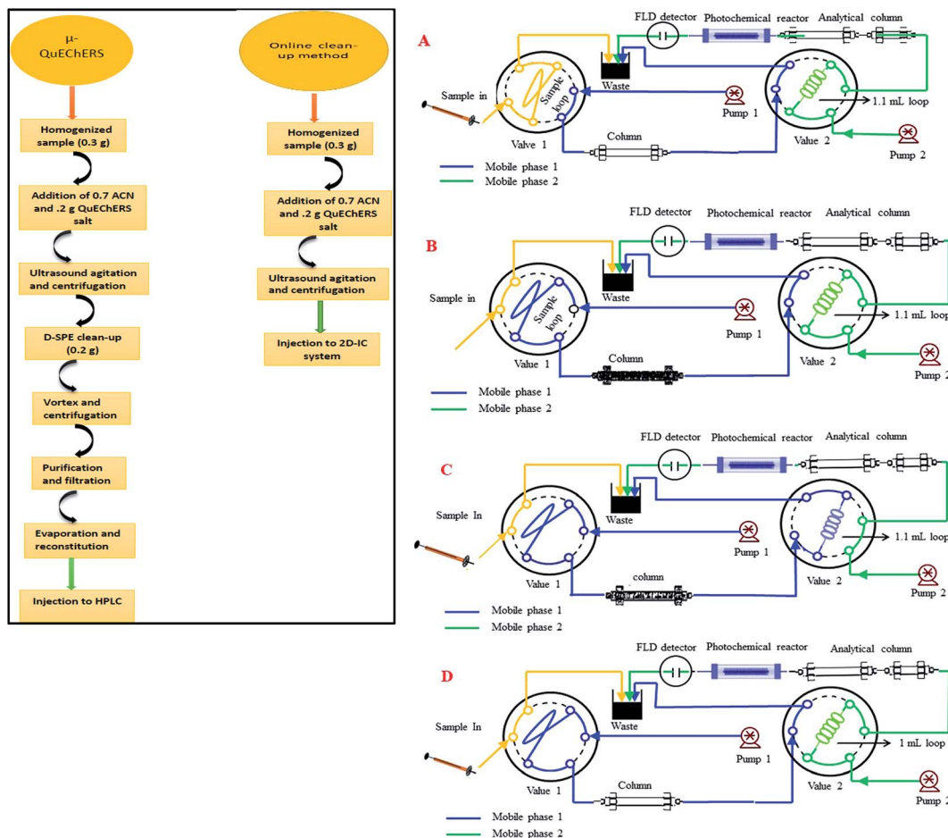
Fig. 2 Systematic flow scheme of 2D-IC system: (A) sample loading; (B) matrix interferences removal; (C) analytes transfer in second dimension and (D) regeneration, re-equilibrium of pre-treatment column and isocratic separation and post column PIF detection in second dimension.
