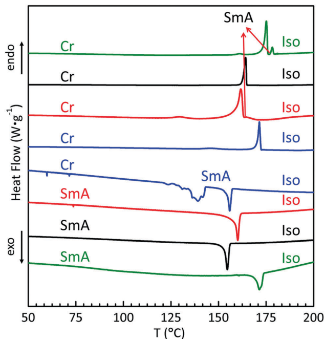
Fig. 1 DSC thermograms of trans-C 0 -Chol (green lines), trans-C 1 -Chol (black lines), trans-C 3 -Chol (red lines) and trans-C 5 -Chol (blue lines) upon the first heating (4 upper curves) and first cooling (4 lower curves) cycle at a rate of 2 °C min −1 . Samples are solids obtained by recrystallization after synthesis.
