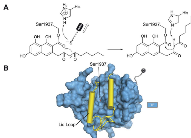
Fig. 15 The PksA TE domain. (A) Proposed reaction mechanism and product release. (B) TE domains have a lid loop that closes the active site.
